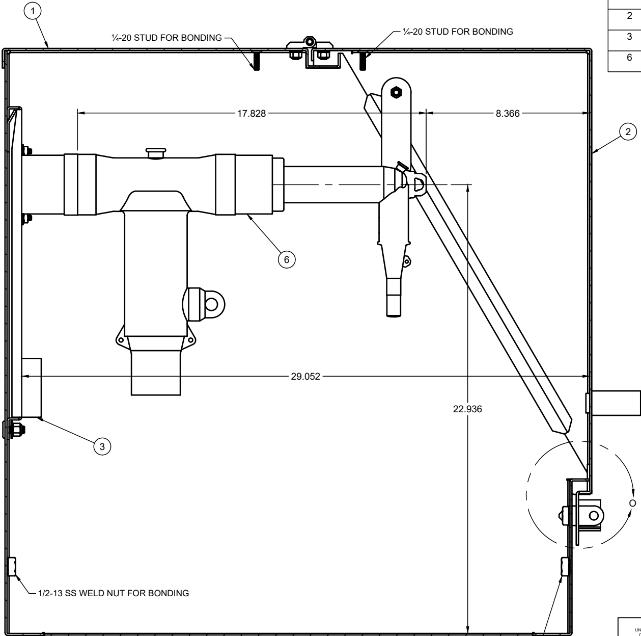
SECTION K-K SCALE 1:5
